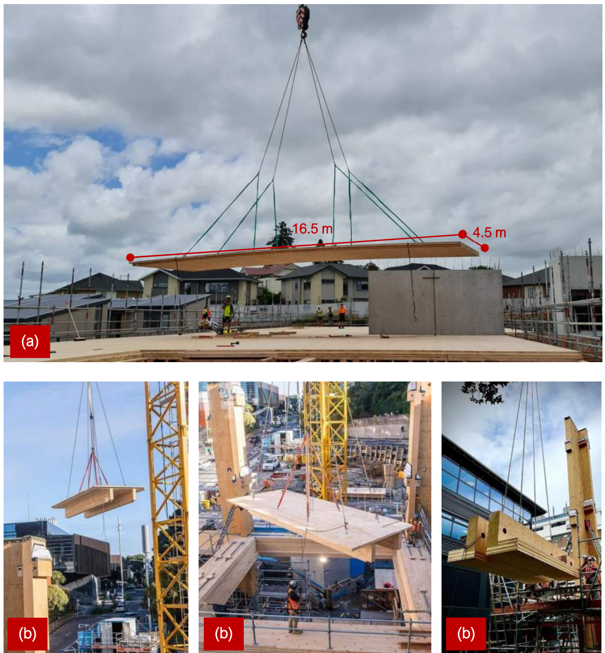
Figure 17: Examples lifting solutions for Red Stag EWPs; (a) Installation shows an example of a 75 square meter Red Stag CLT panel being effortlessly installed on site. 16.5 m x 4.5 m Red Stag CLT floor panel is lifted via eight screw anchor lifting points; (b) Red Stag CLT composite element lifting.
