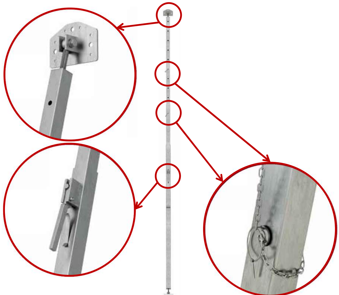
Figure 83: Components of a GIRAFFE prop [19] .
