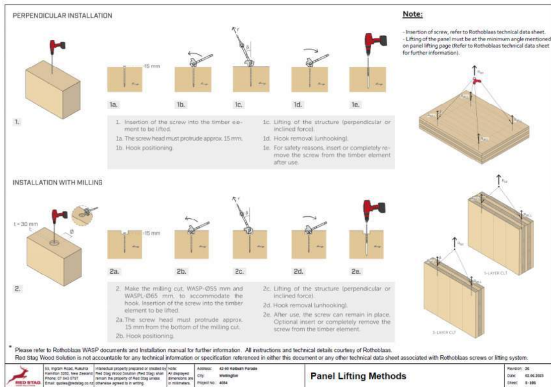
Figure 11: Example of lifting system option (client must confirm acceptance).
