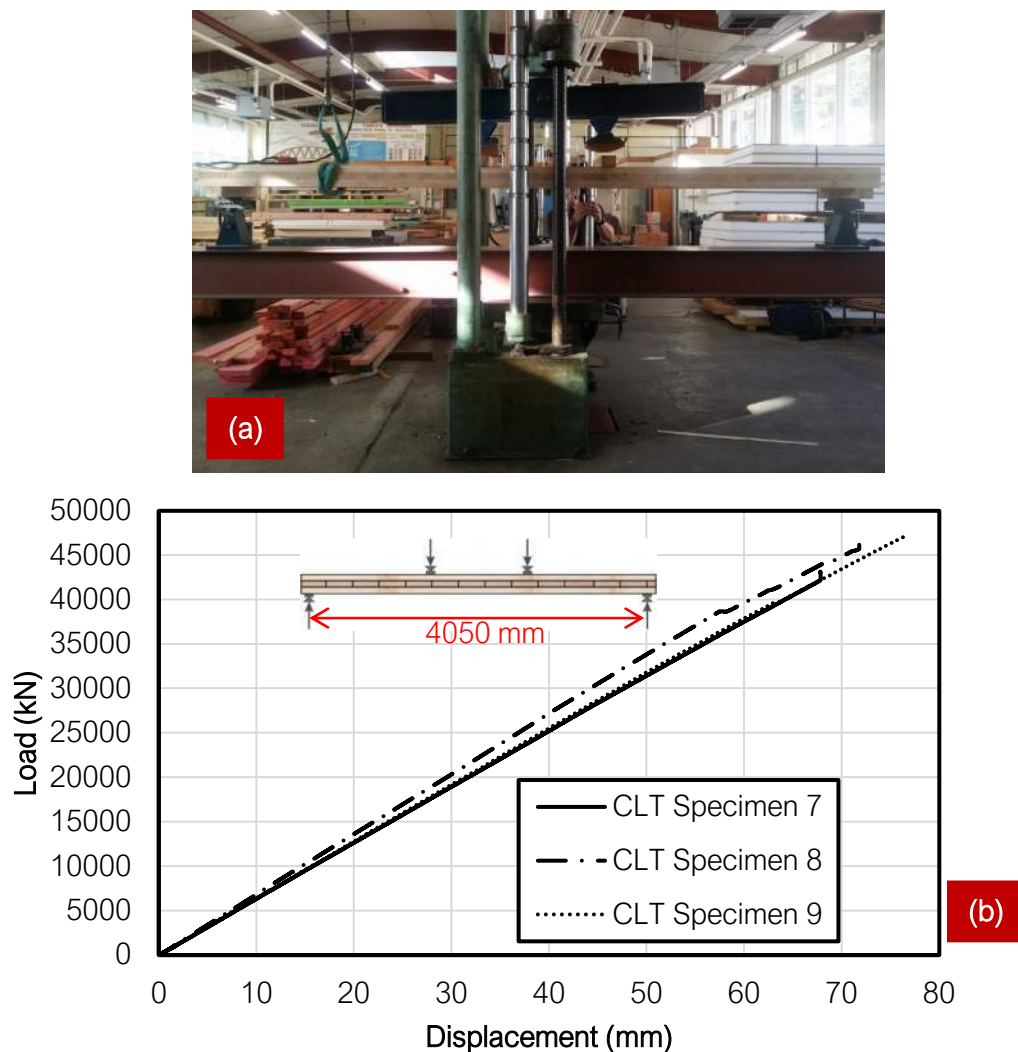
Figure 61: Bending Test; a) Test setup for 135 mm thick Red Stag CLT Panel (Support to support span = 4050 mm); b) Load deflection diagram based on the recorded data by SCION.
