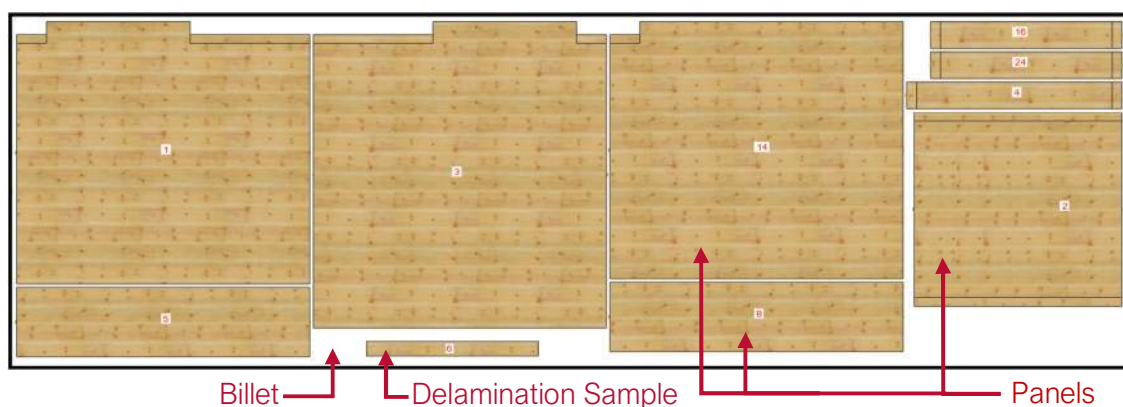
Figure 3: Red Stag CLT billet with nested panels.
