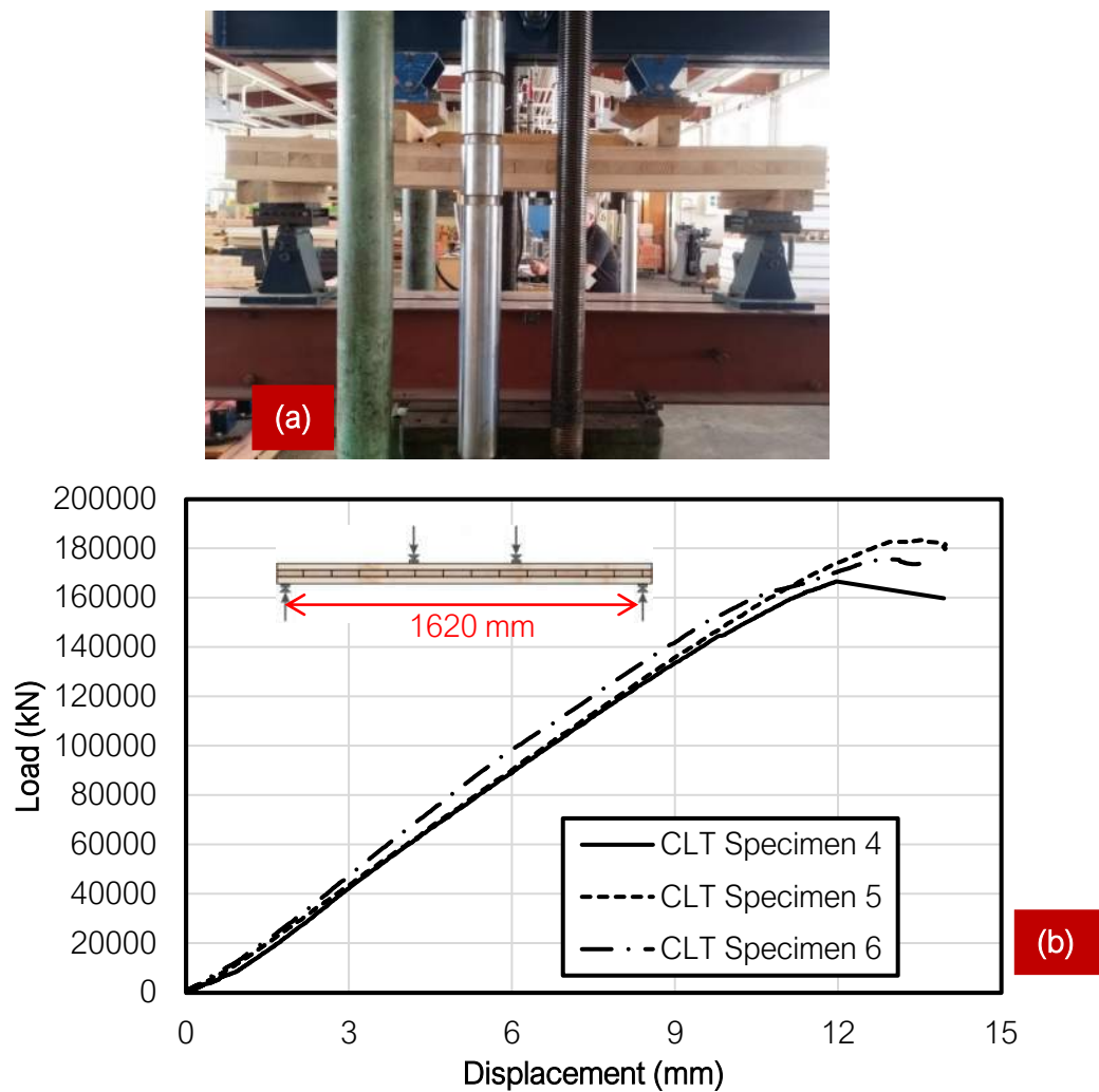
Figure 60: Rolling Shear Strength and Stiffness Test; a) Test setup for 135 mm thick Red Stag CLT Panel (Support to support span = 1620 mm); b) Load deflection diagram based on the recorded data by SCION.
