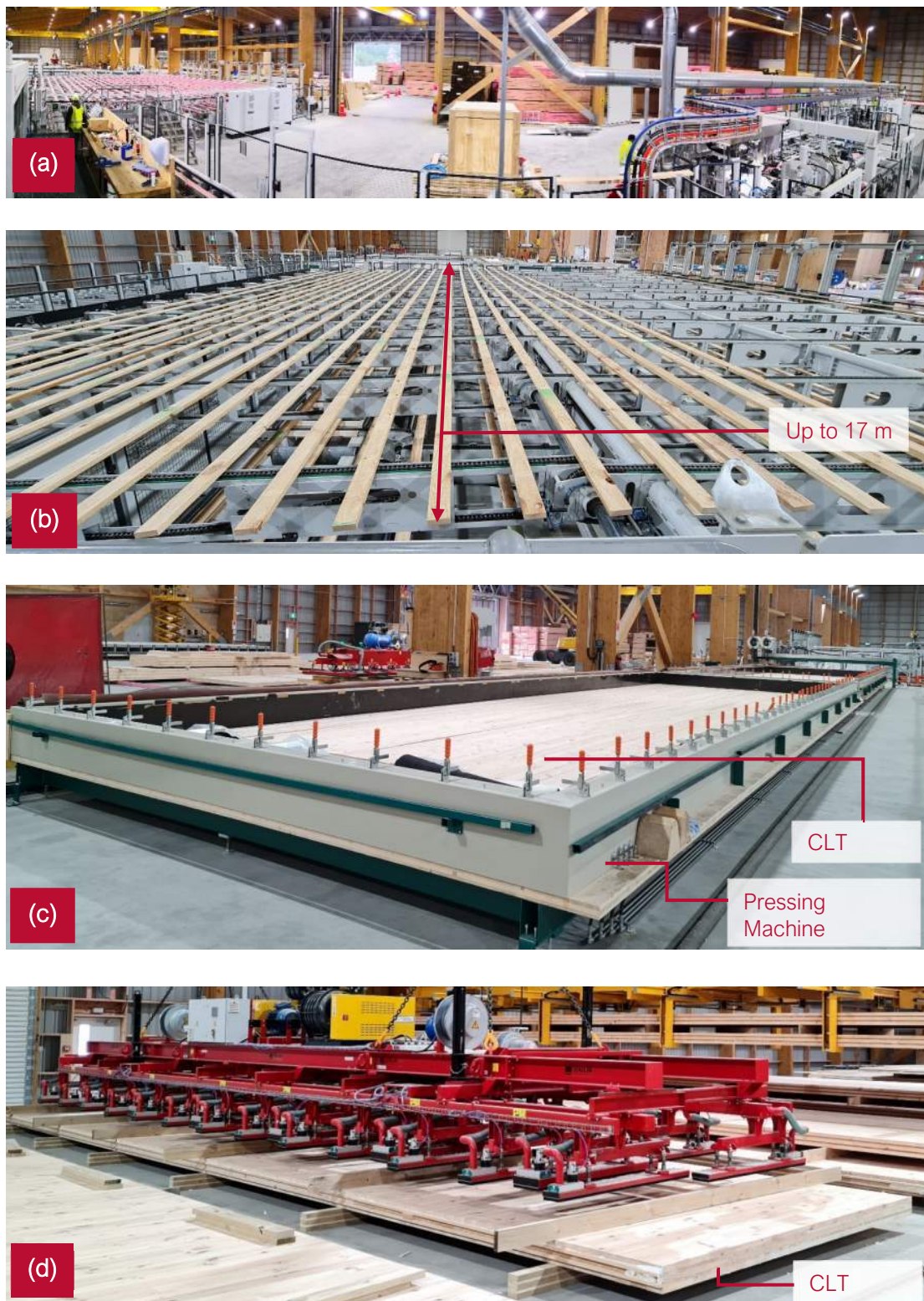
Figure 48: Red Stag's Rotorua EWP manufacturing facility; a) panoramic view of the remanufacturing line; (b) 16.5 meter lamella out of the Finger Joints (FJ) line; (c) EWP laminating equipment; (d) EWP material handling equipment.
