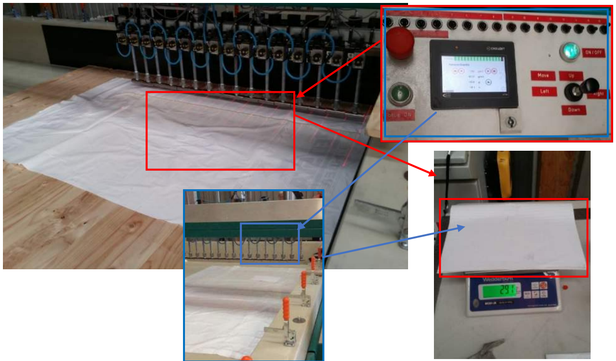
Figure 53: Laminating glue application rate QA management ( \text{g/m}^2 ).
