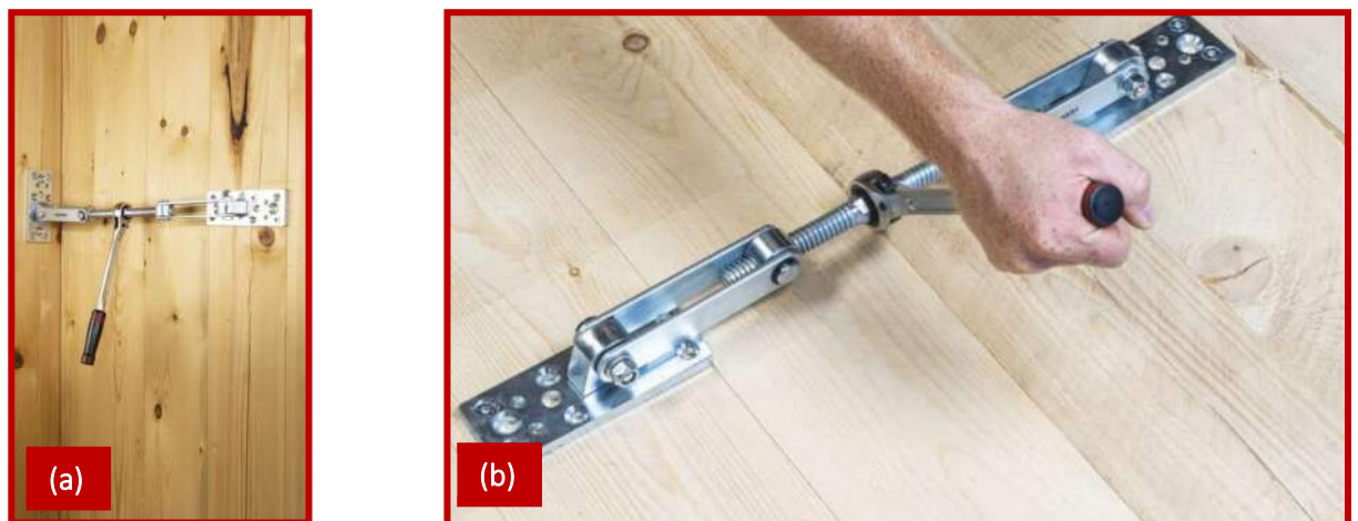
Figure 91: GEKO applications; a) GEKO utilised to pull CLT wall panels together (pulling into a corner); b) GEKO utilised to pull CLT floor panels together [21] .
