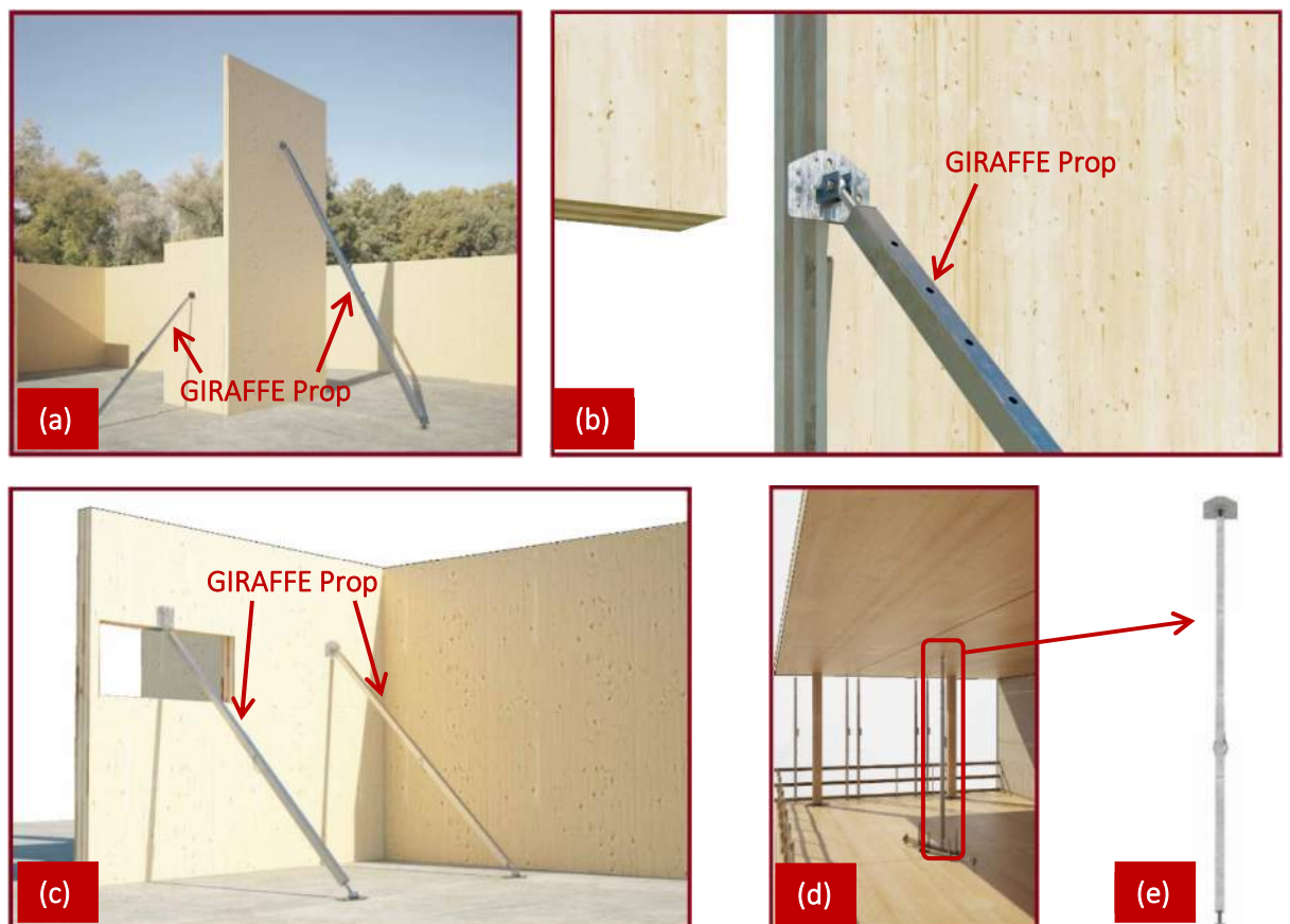
Figure 84: GIRAFFE prop applications in CLT projects; a) GIRAFFE prop for CLT wall installation; b) Application of GIRAFFE prop for wall to wall alignment; c) Application of GIRAFFE prop for wall alignment with opening; d) GIRAFFE prop being utilised in an Acrow prop application for CLT floor support; e) Example of a GIRAFFE prop [19] .
