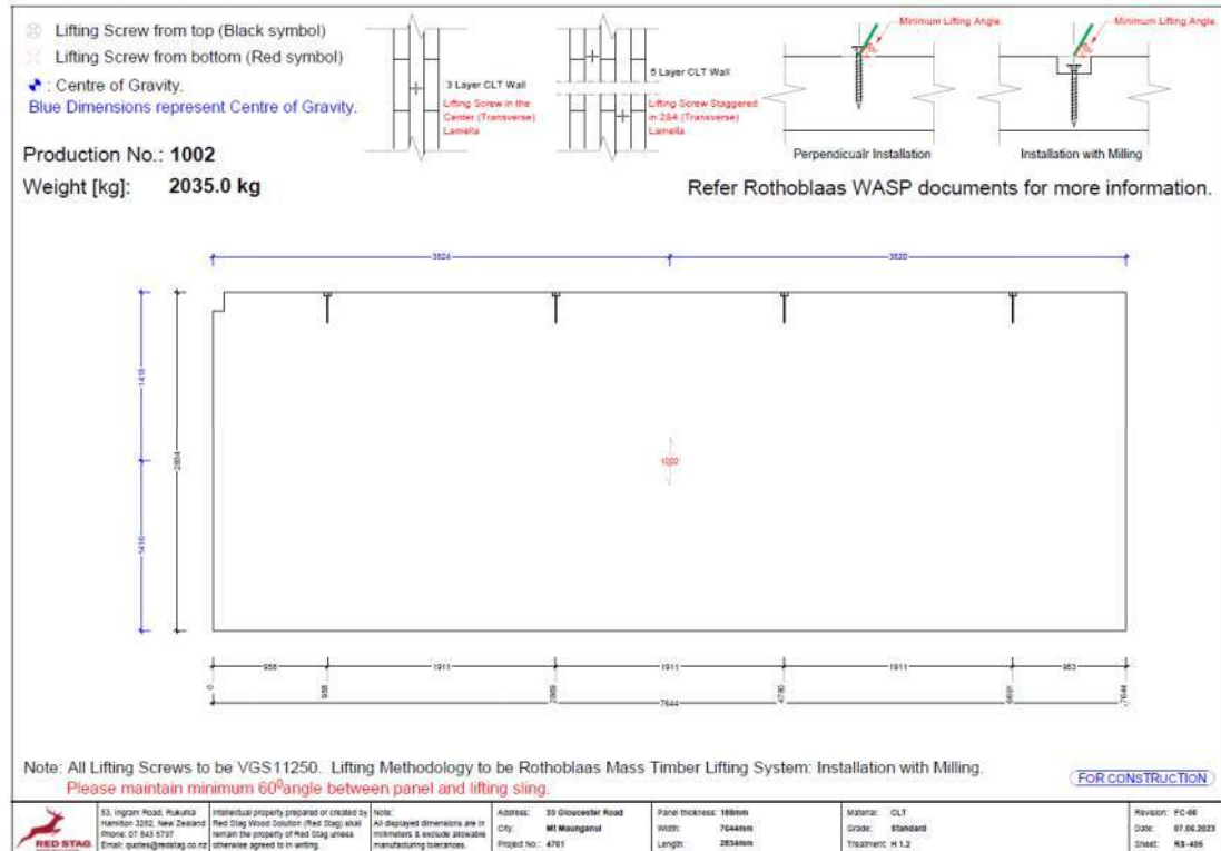
Figure 12: Example of lifting point drawing (Software suggested lift points - Client to confirm).
