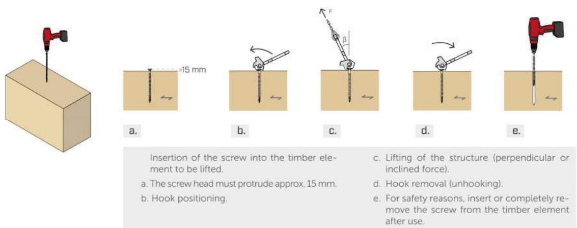
Figure 24: Inclined WASP installation without milling [1] .
