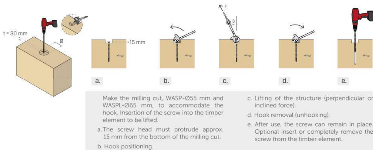
Figure 22: WASP installation with milling [1] .
