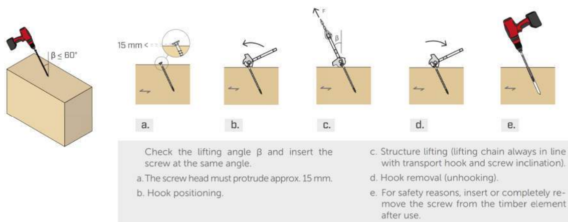
Figure 23: Perpendicular WASP installation without milling [1] .
