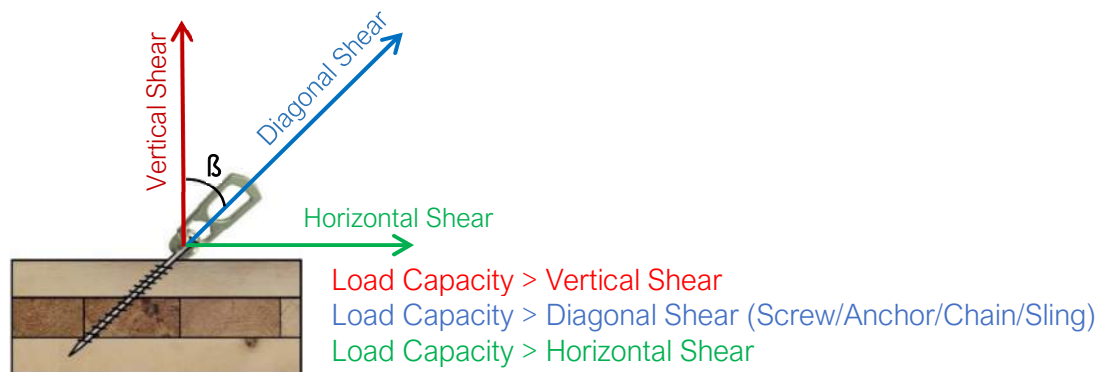
Figure 19: Lifting capacity reduction based on angle of lift.
