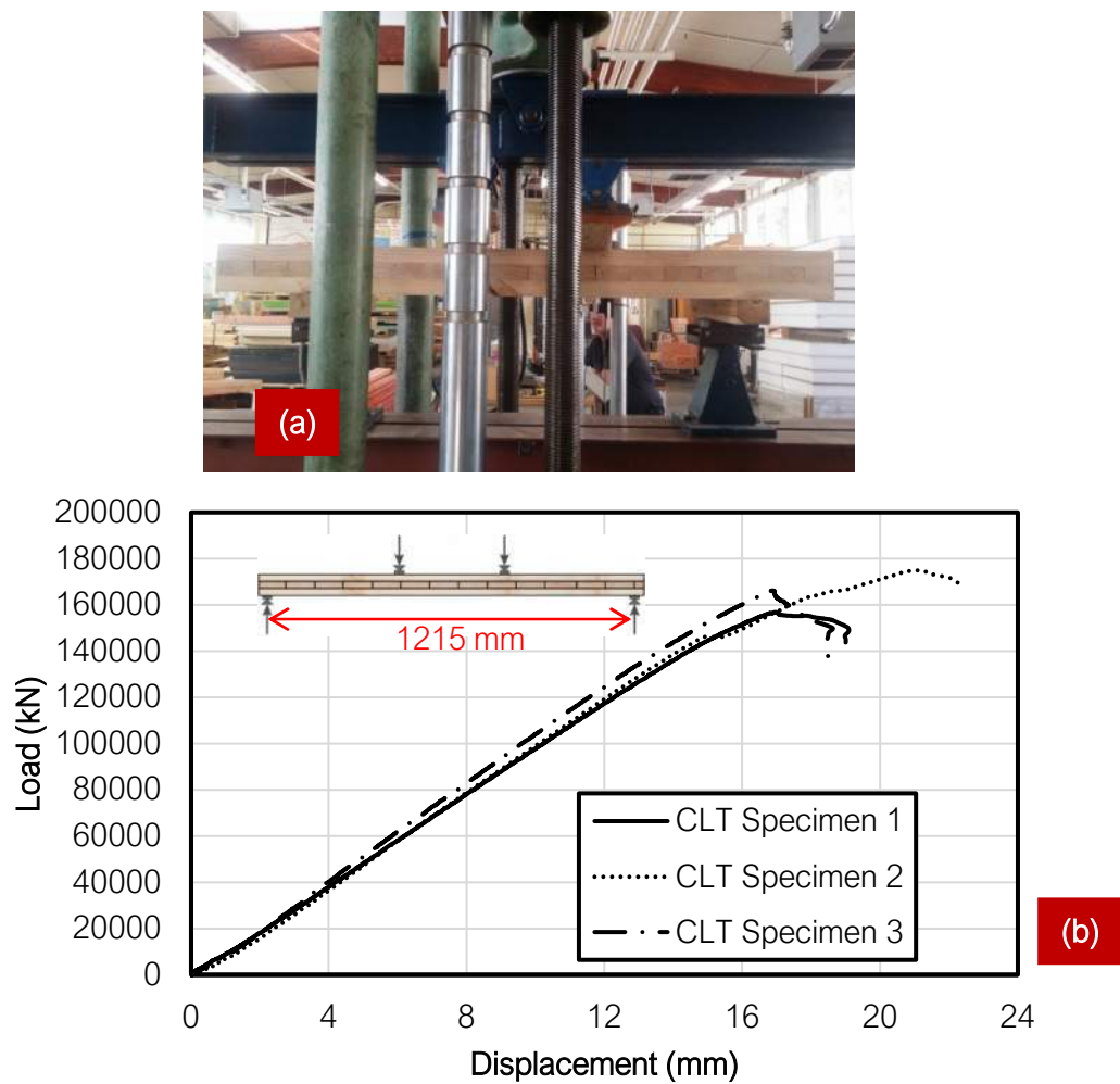
Figure 59: Rolling Shear Strength Test; a) Test setup for 135 mm thick Red Stag CLT Panel (Support to support span = 1215 mm); b) Load deflection diagram based on the recorded data by SCION.
