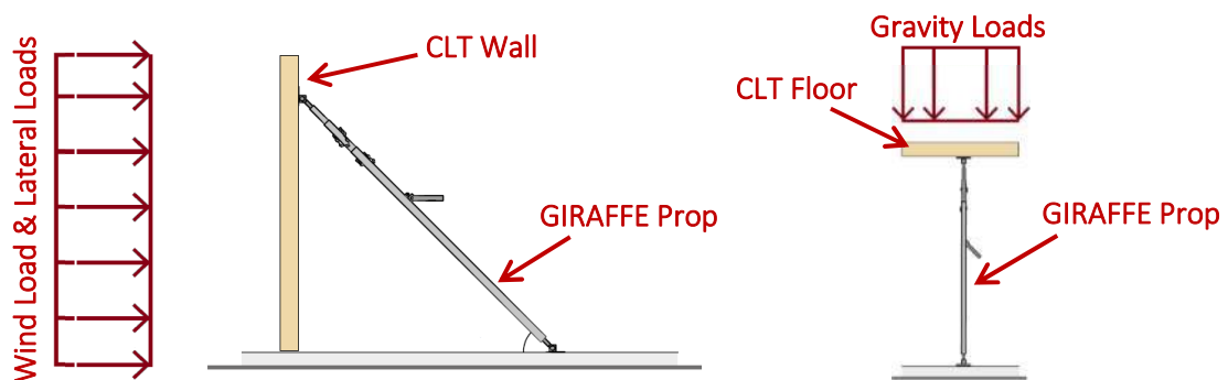
Figure 87: Loadings that need to be consider for GIRAFFE prop calculation [19] .
